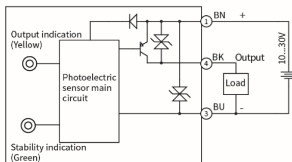
PNP
