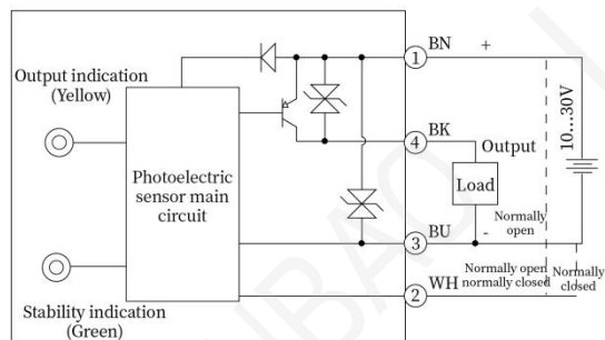
PNP
